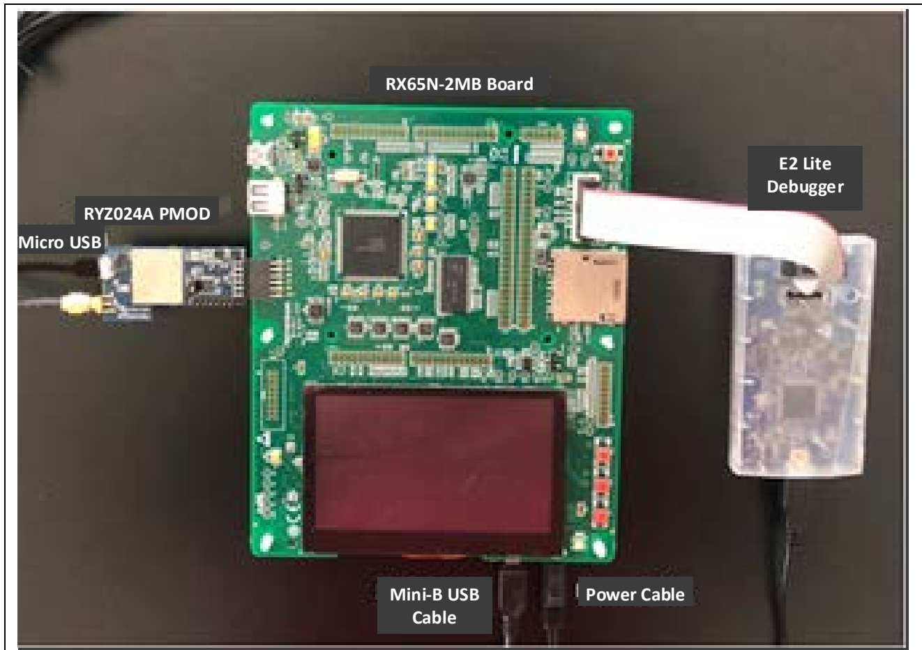
Figure 1. RSK-RX65N-2MB Setup with RYZ024A PMOD Board Connected
