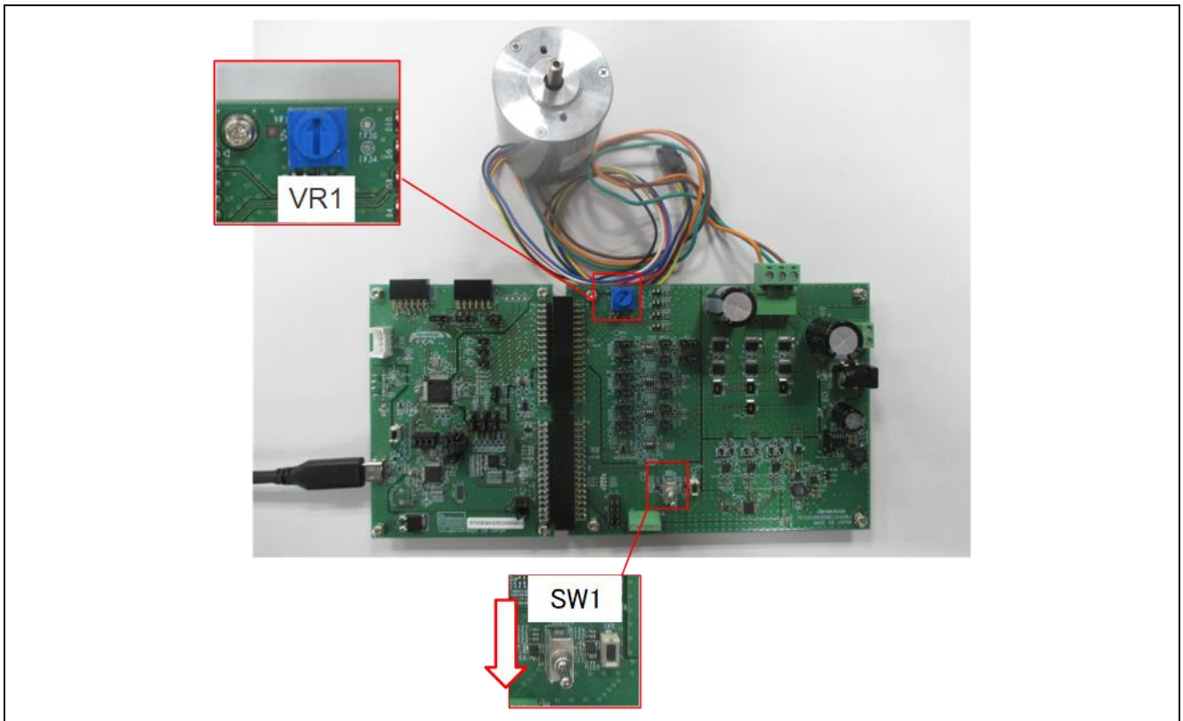
Figure 4-3 Hardware configuration
