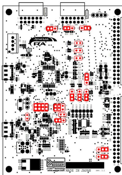
Figure 4-2 Jumper pin setting of CPU Board
