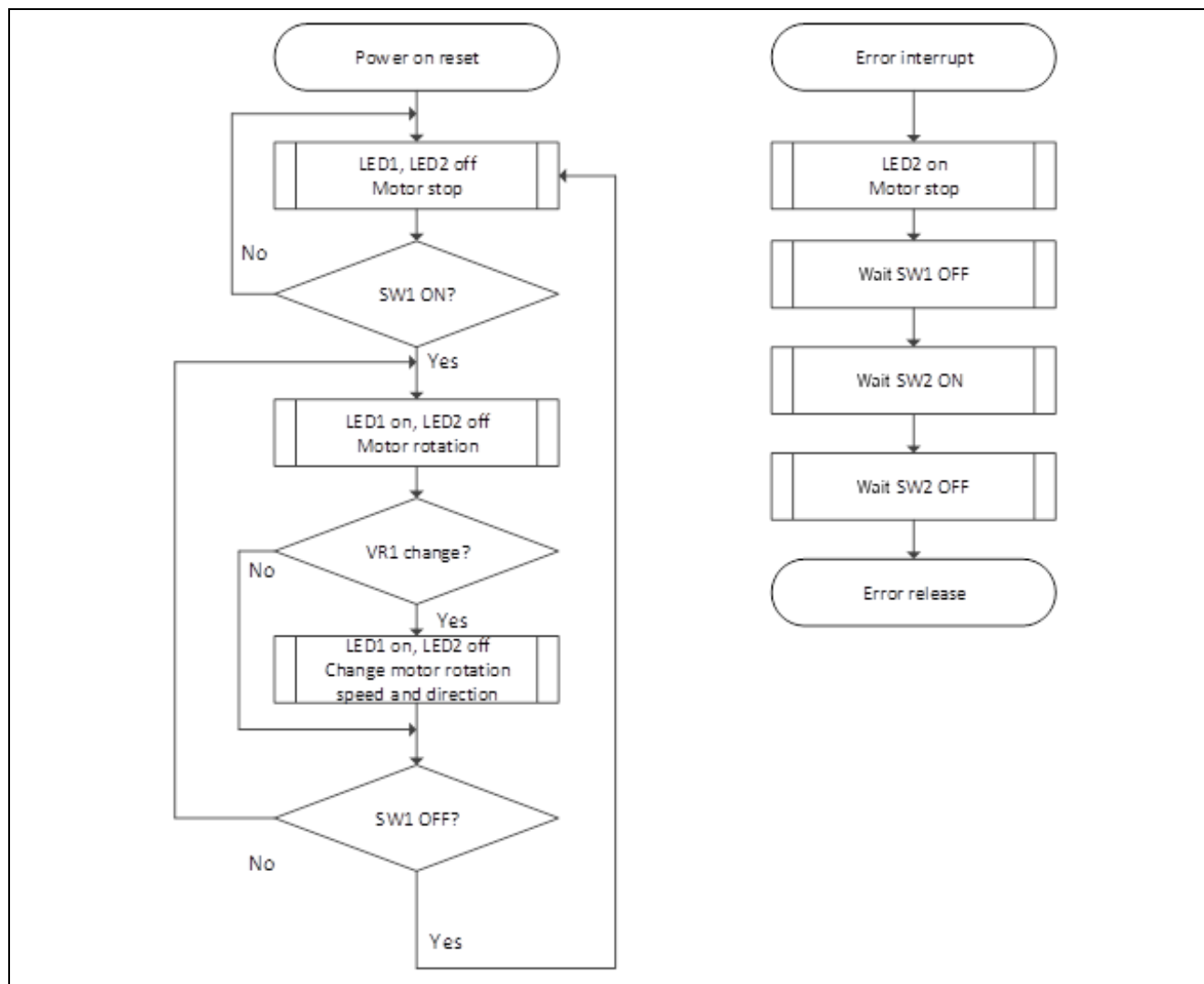
Figure 3-1 Quick start sample project flow
