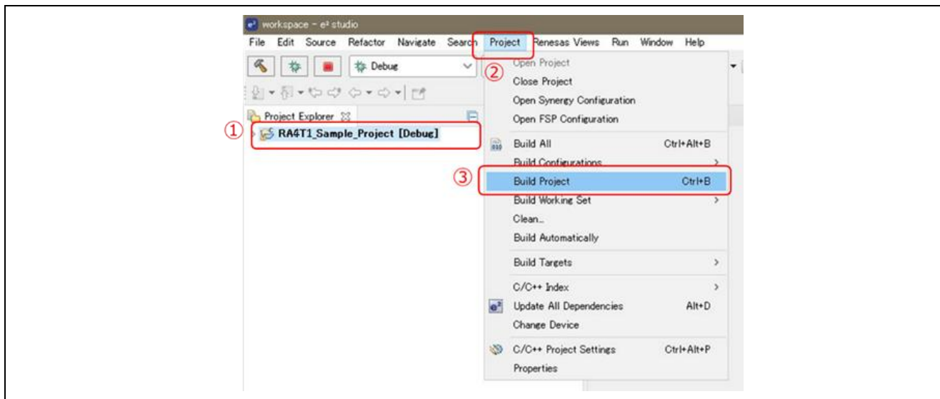
Figure 5-4 Build project
