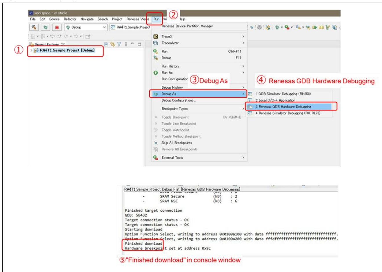
Figure 5-5 Flash programming
