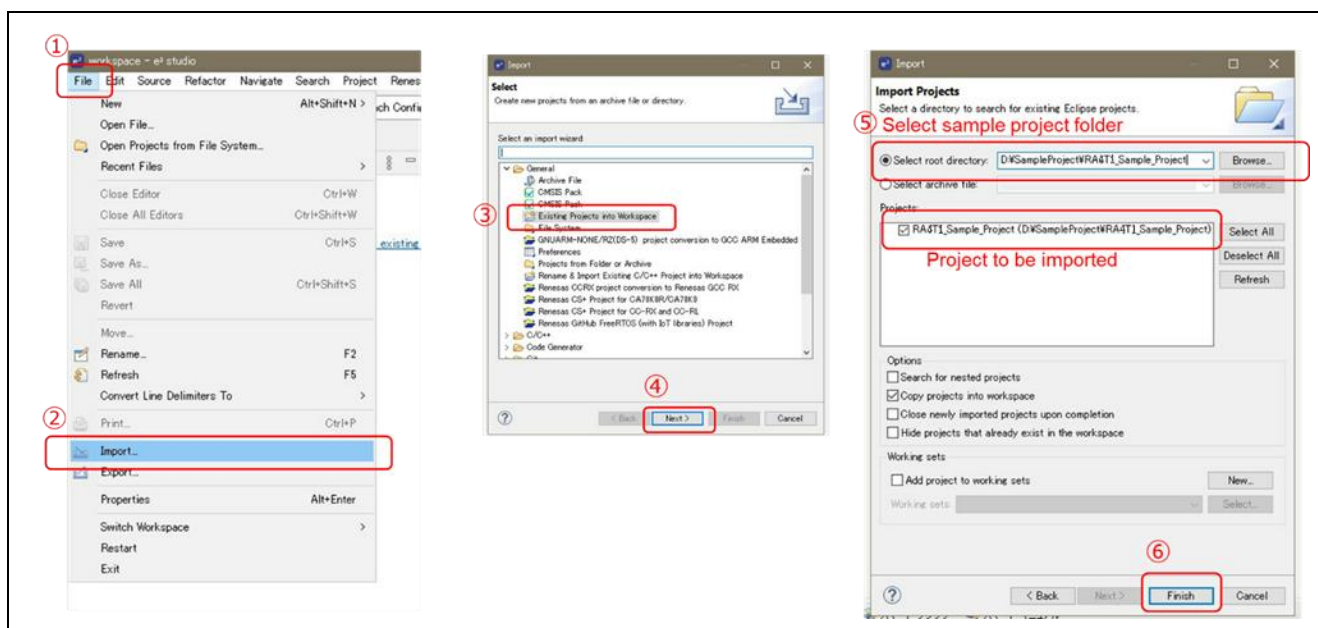
Figure 5-2 Import project
