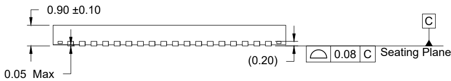
SIDE VIEW
