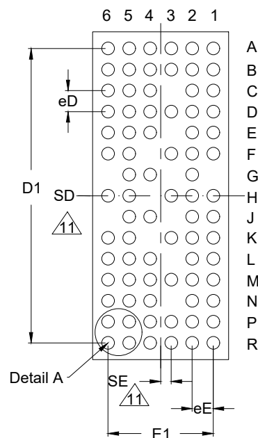
Bottom View
