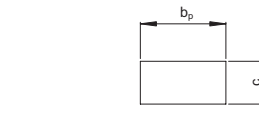
Terminal cross section (Ni/Pd/Au plating)
