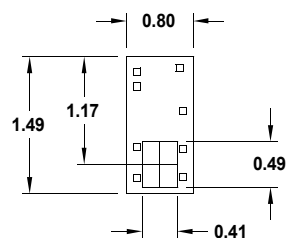
DETECTOR DIMENSION
