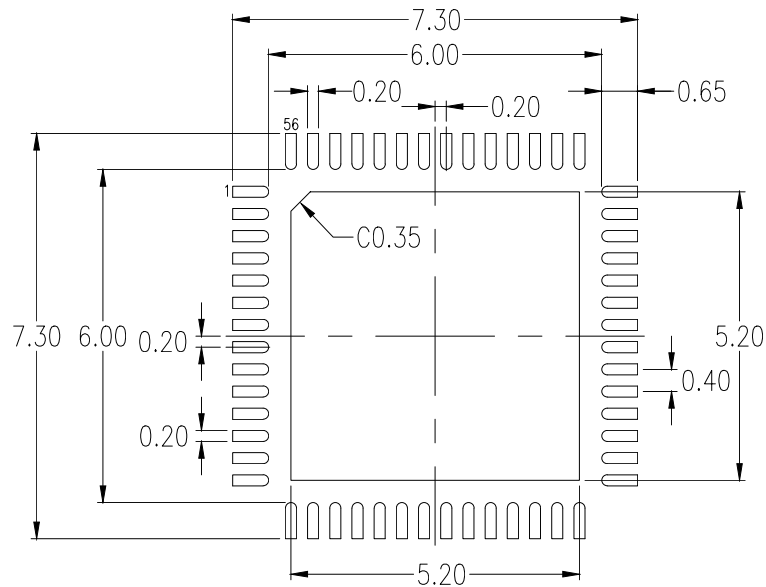
RECOMMENDED LAND PATTERN DIMENSION
