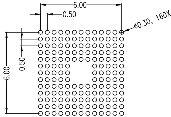
RECOMMENDED LAND PATTERN DIMENSION
