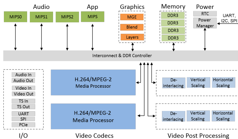
Figure 1: Device diagram
