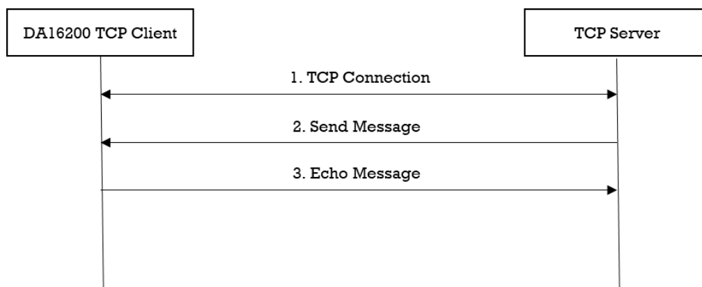
Figure 15: Workflow of TCP Client
