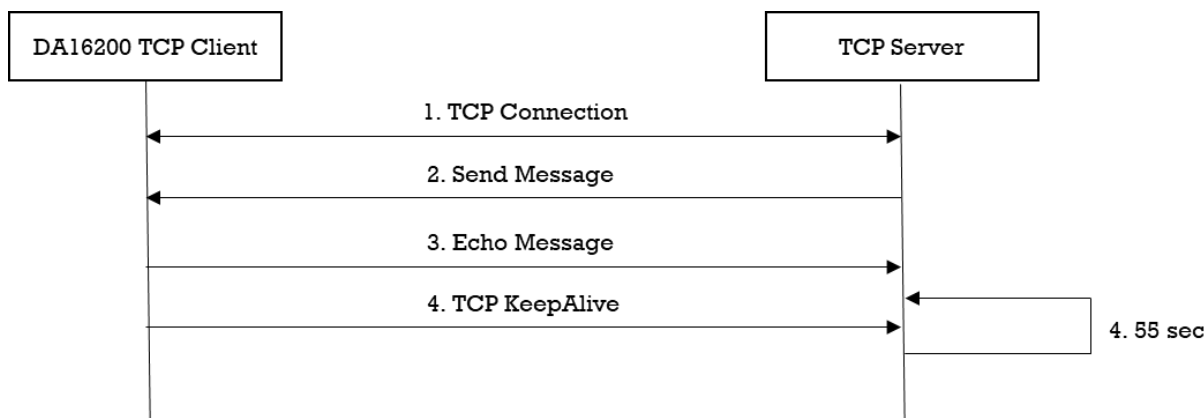
Figure 19: Workflow of TCP Client with KeepAlive
