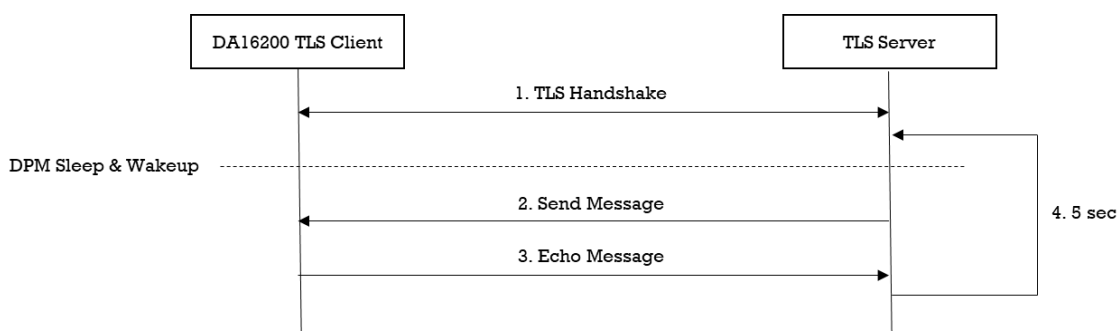
Figure 32: Workflow of TLS Client in DPM
