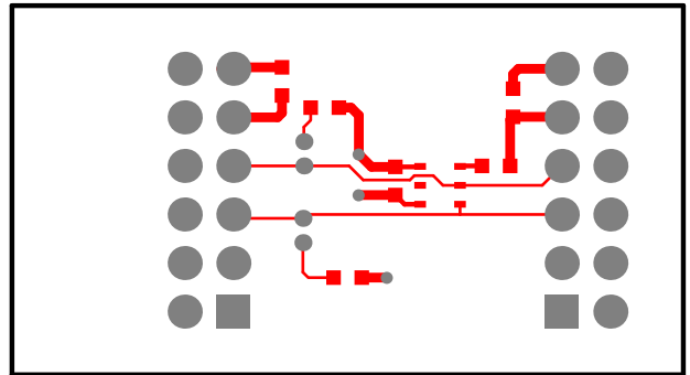
Figure 7. Copper Top
