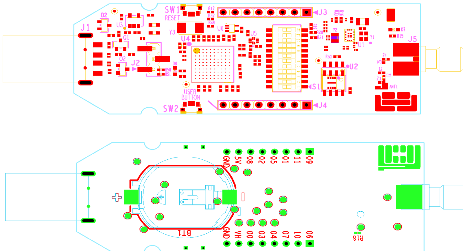
Figure 31. Components placement, top side on the left and bottom side on the right
