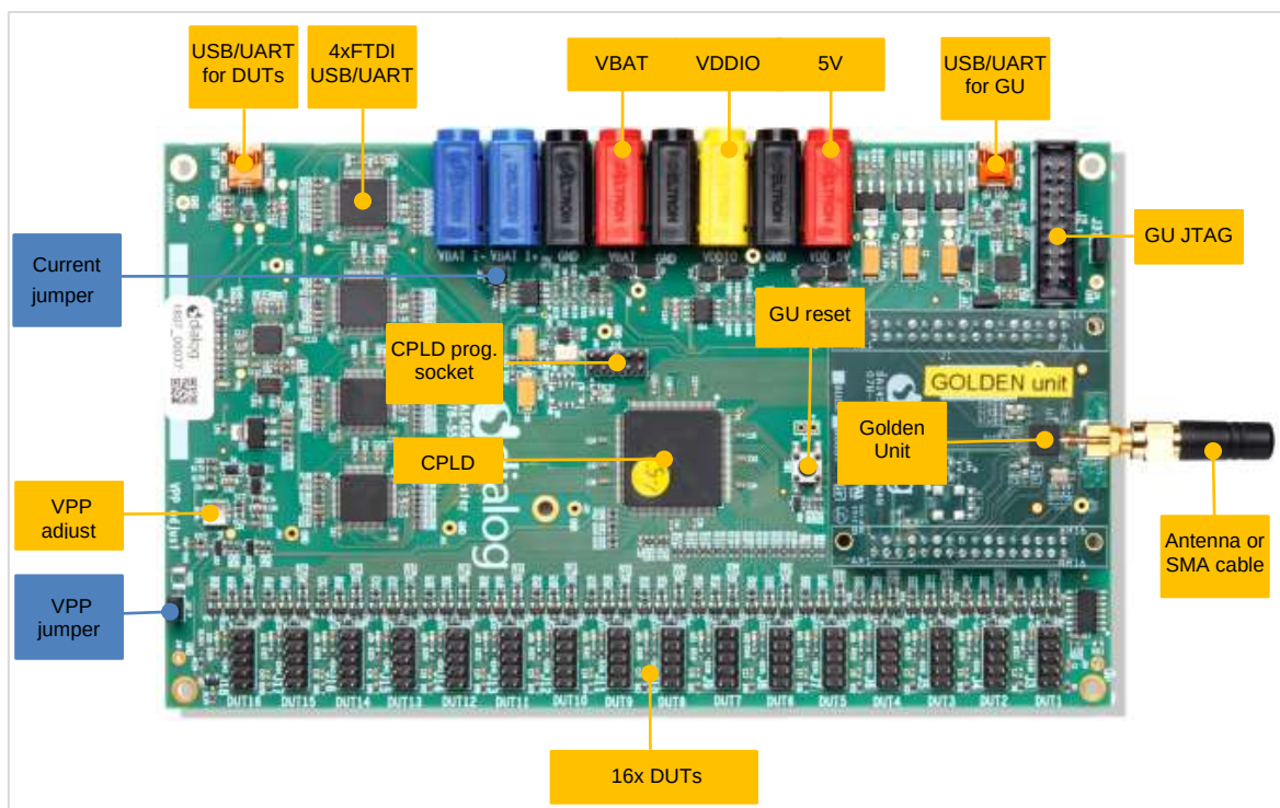
Figure 3: Top view of the PLT hardware board
