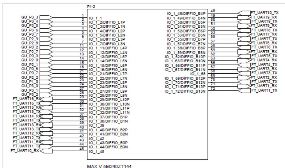
Figure 146: CPLD FTDI and GU control connections
