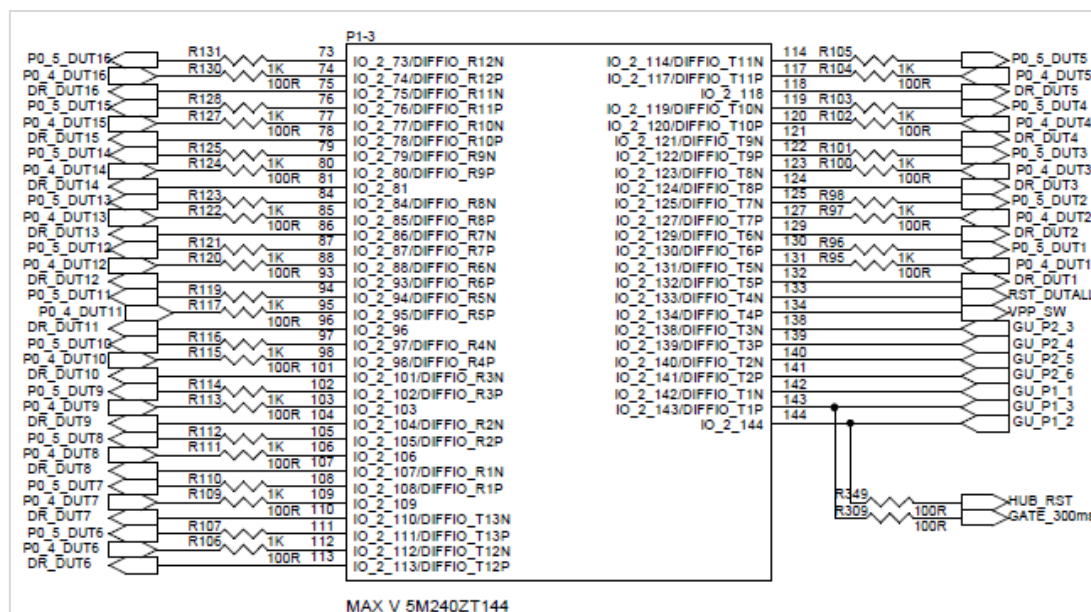
Figure 145: CPLD DUT UART connections
