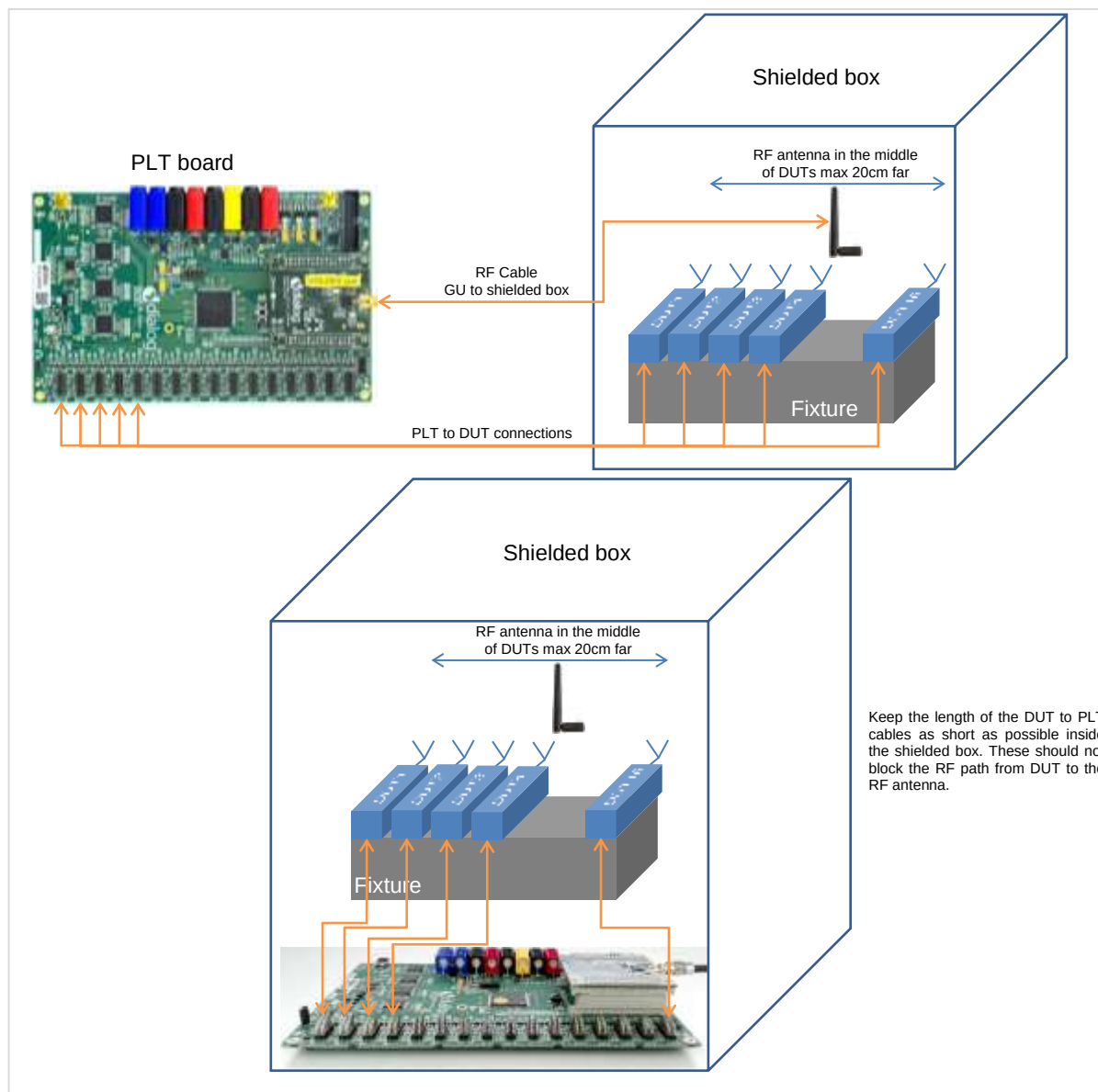
Figure 156: Setup diagram
