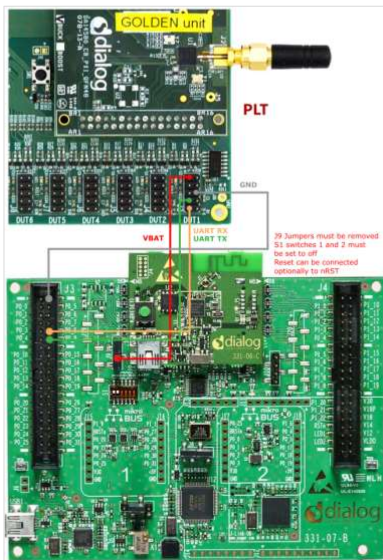
Figure 166 DA1469x DK Pro Motherboard PLT connection
