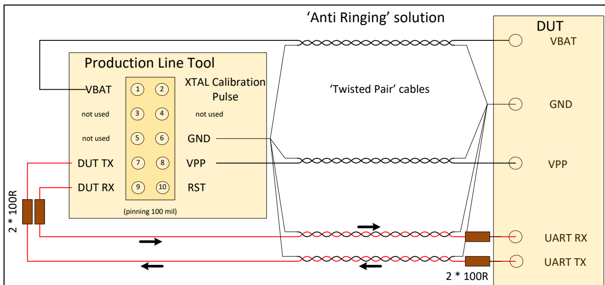
Figure 163: Anti-ringing solution
