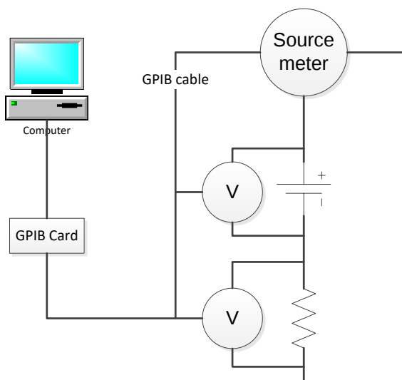
Figure 11: Hardware setup for Battery Profiling Option
