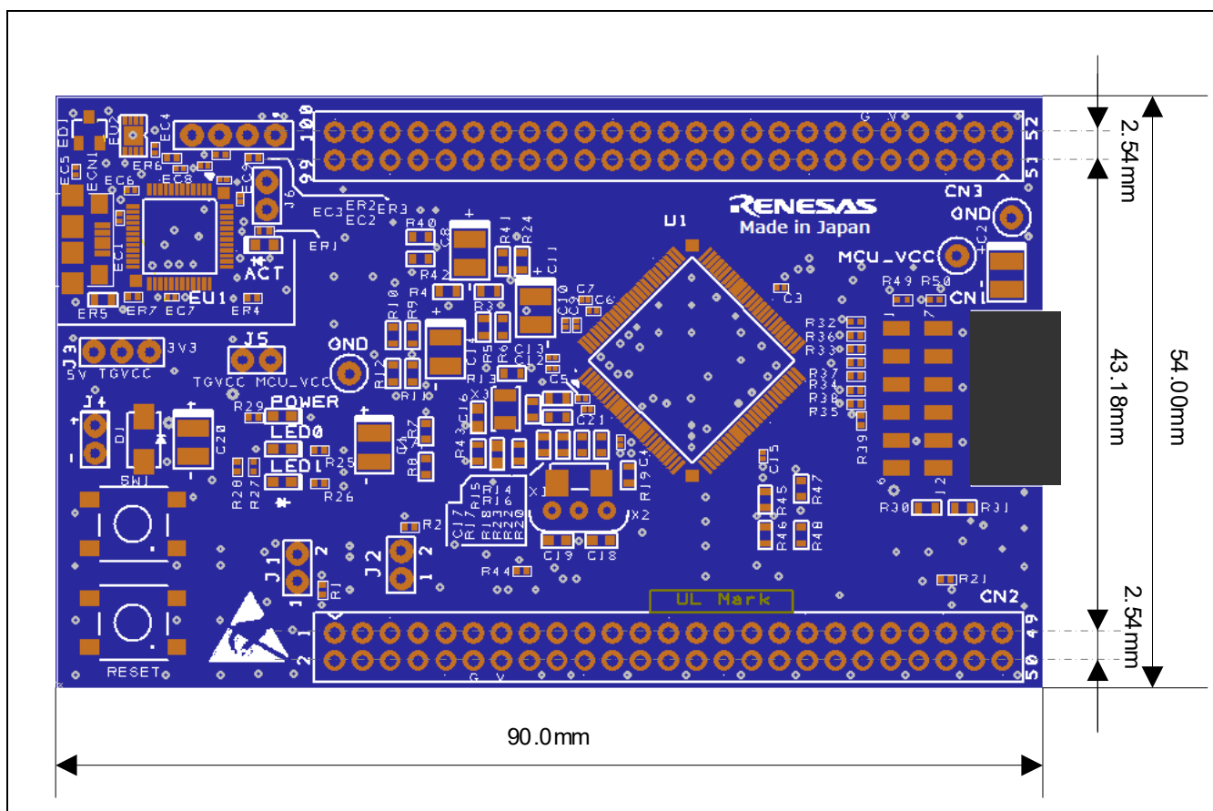
Figure 3-1 Parts Layout
