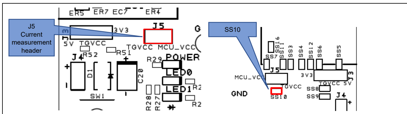
Figure 5-4 Positions of the Current Measurement Header (J5) (Top Side) &amp; Pattern for Cutting (SS10) (Soldered Side)
