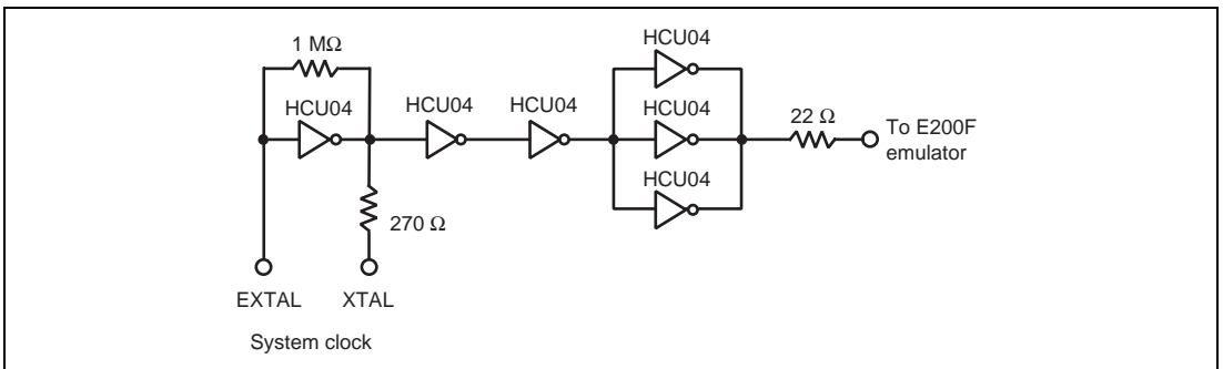
Figure 8 Clock Oscillator
