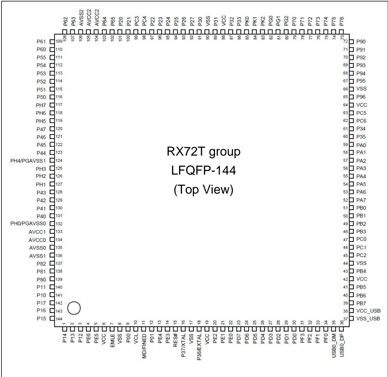
Figure 6.1 RX72T Pin Assignments
