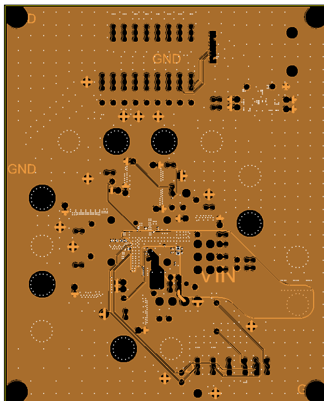
Figure 20. Layer 5 Copper
