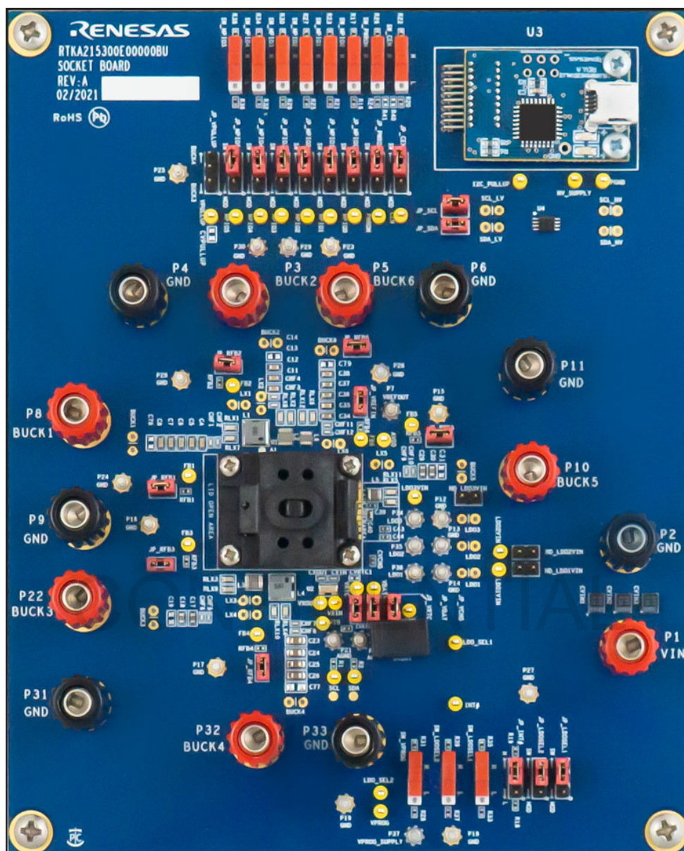
Figure 12. RTKA215300E00000BU Evaluation Board (Top)
