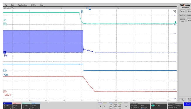
Figure 16. Shutdown by EN at 1A Load
