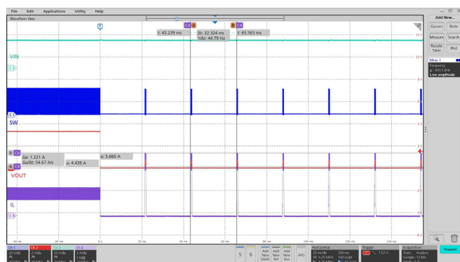
Figure 17. Overcurrent Protection
