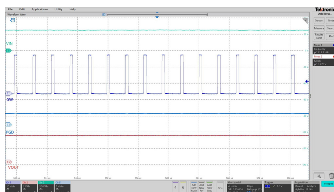
Figure 13. Steady State at 2A Load
