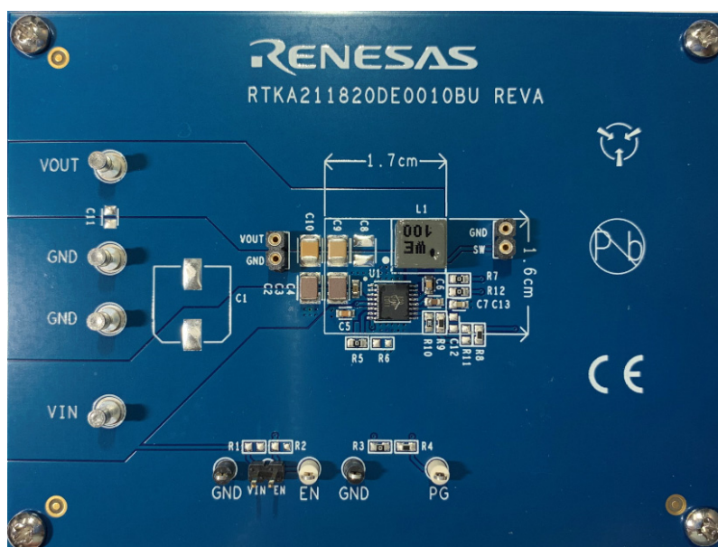
Figure 3. RTKA211820DE0010BU Evaluation Board (Top)
