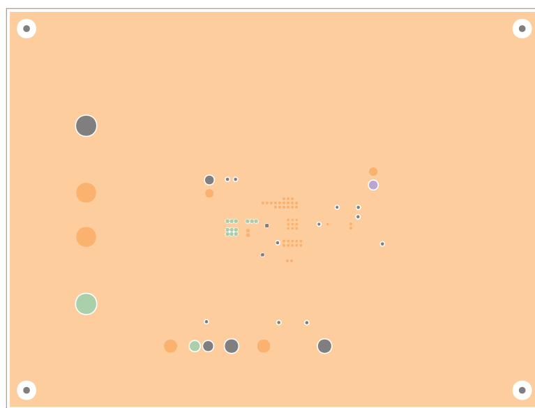
Figure 7. Second Layer
