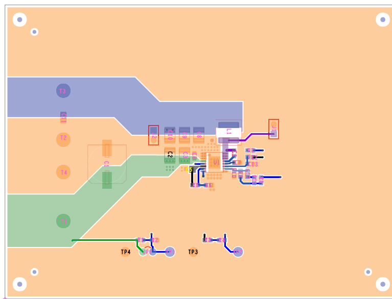
Figure 6. Top Layer
