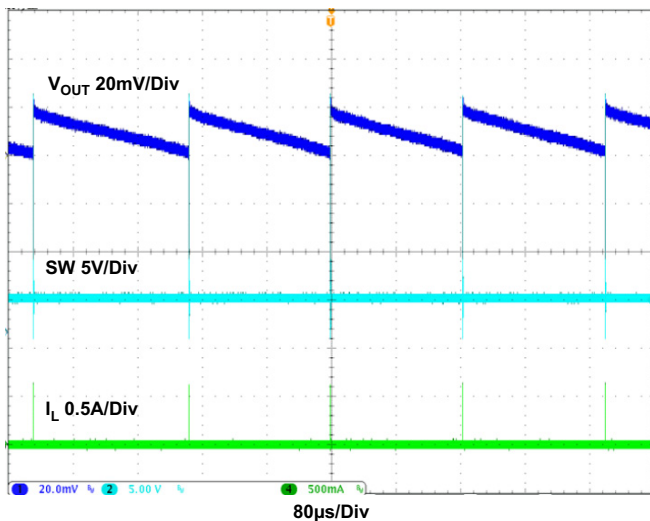
Figure 12. Output Ripple at No Load
