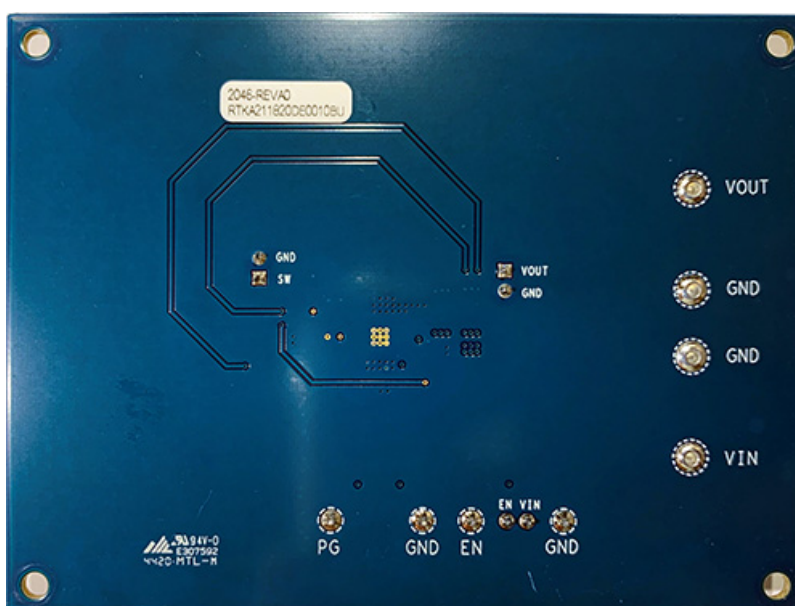
Figure 4. RTKA211820DE0010BU Evaluation Board (Bottom)
