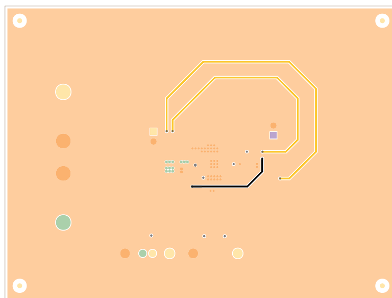
Figure 9. Fourth Layer
