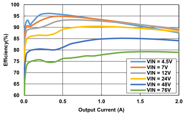
Figure 10. Efficiency vs Load
