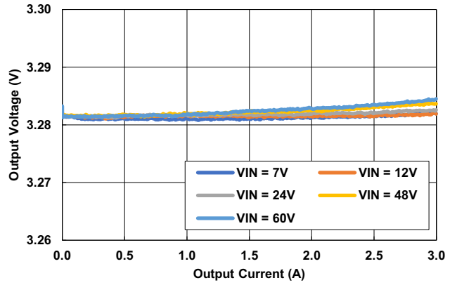
Figure 10. Load Regulation
