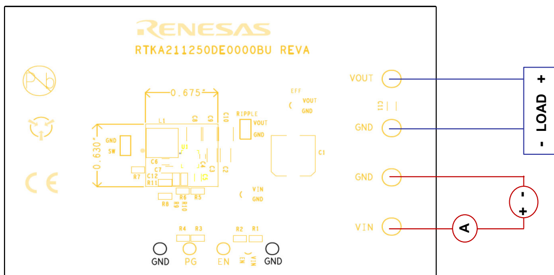
Figure 2. RTKA211250DE0000BU Board Setup
