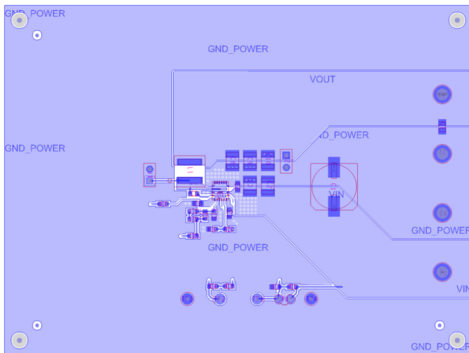
Figure 5. Top Layer
