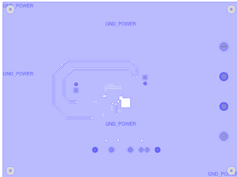
Figure 8. Bottom Layer
