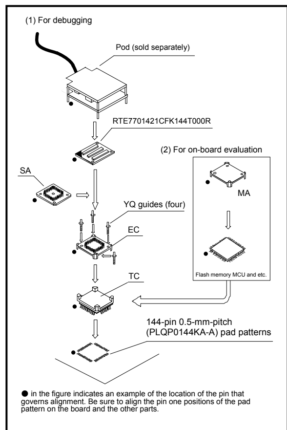
Figure 2 Usage of the RTE7701421CFK144T000R
