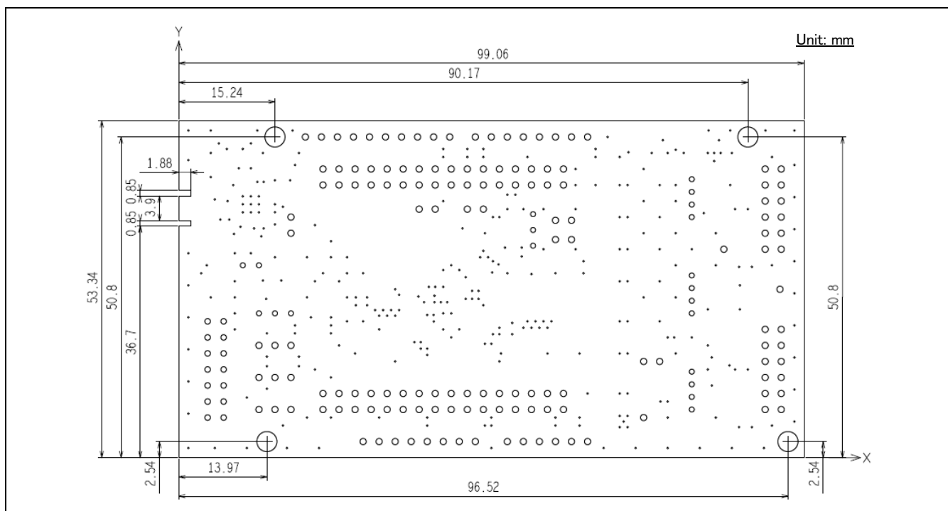
Figure 3-2 External Dimensions
