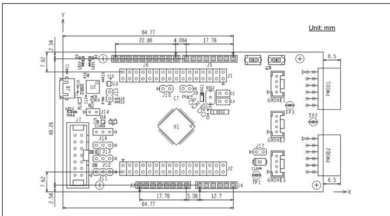
Figure 3-1 Parts Layout
