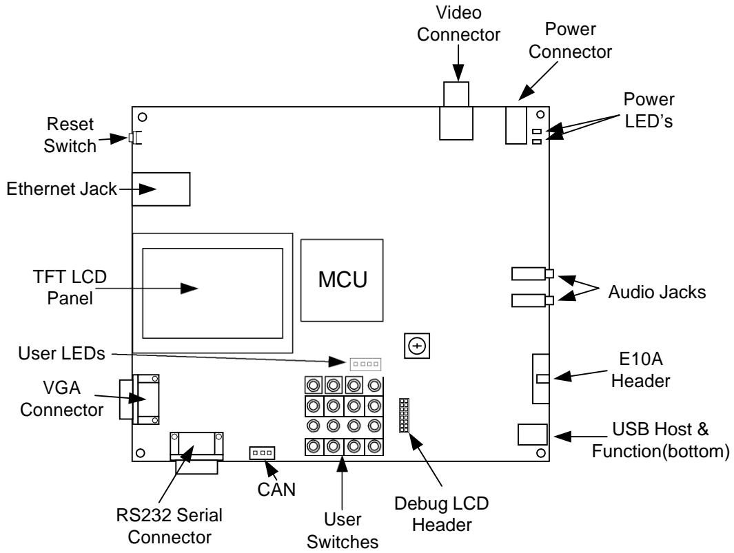
Figure 4-1: Board Layout
