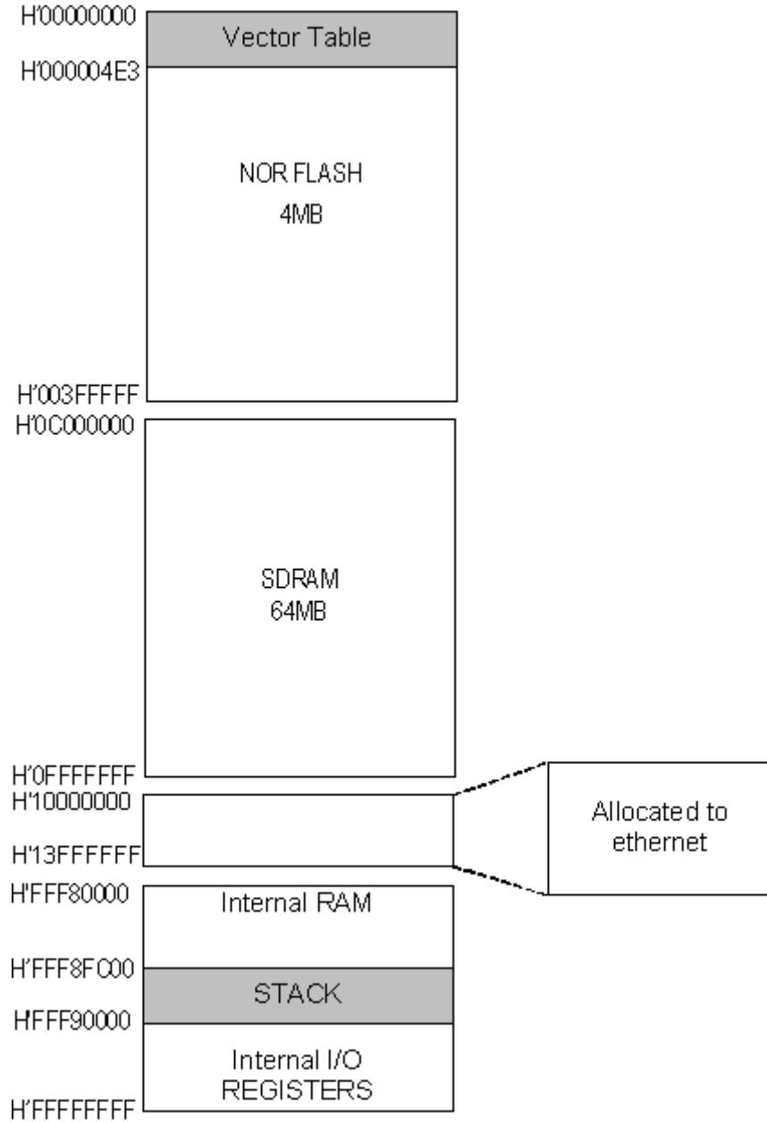
Figure 10-1: RSPSH7267 Memory Map
