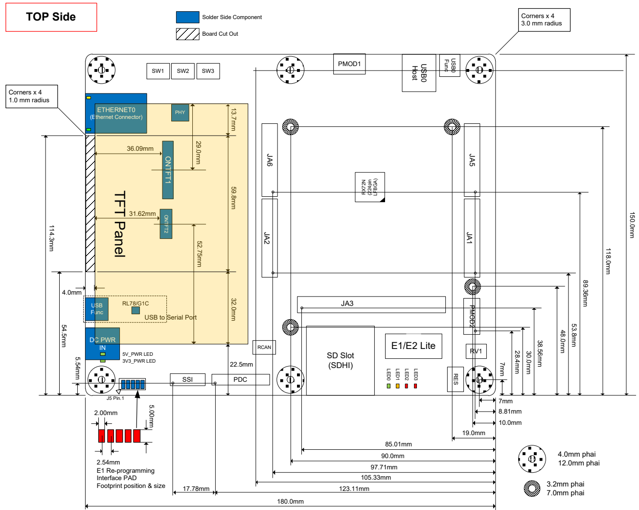
Figure 3-2: Board Dimensions
