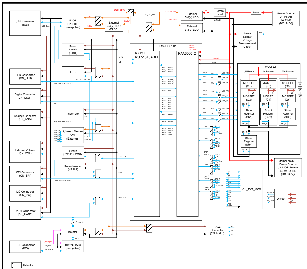
Figure 2-2 Block Diagram
