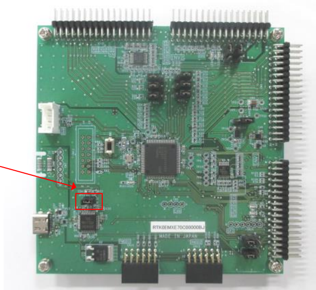
Figure 5-1 Jumper setting of JP11
