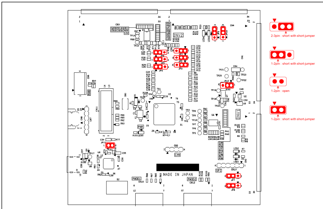
Figure 4-4 Default jumper pin setting
