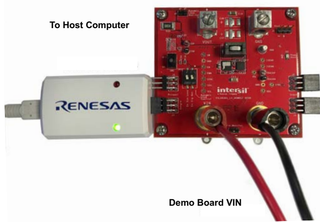
Figure 1. USB to PMBus Typical Set-Up
