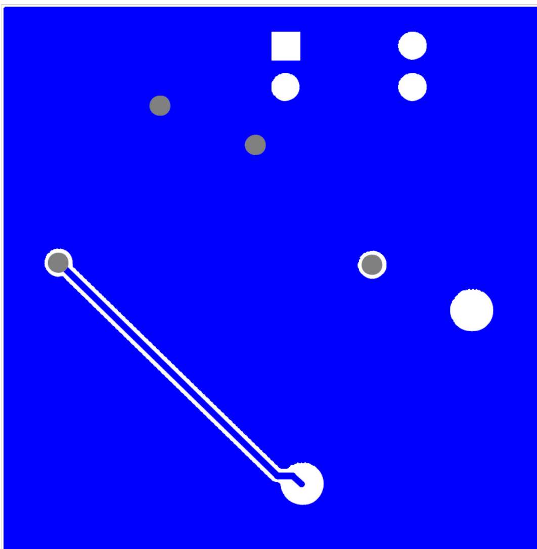
FIGURE 4. BOTTOM LAYER
