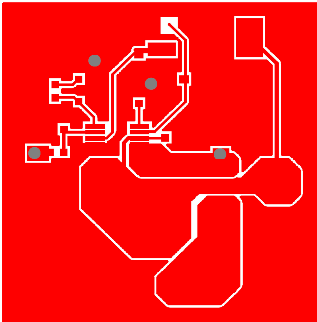
FIGURE 3. TOP LAYER
