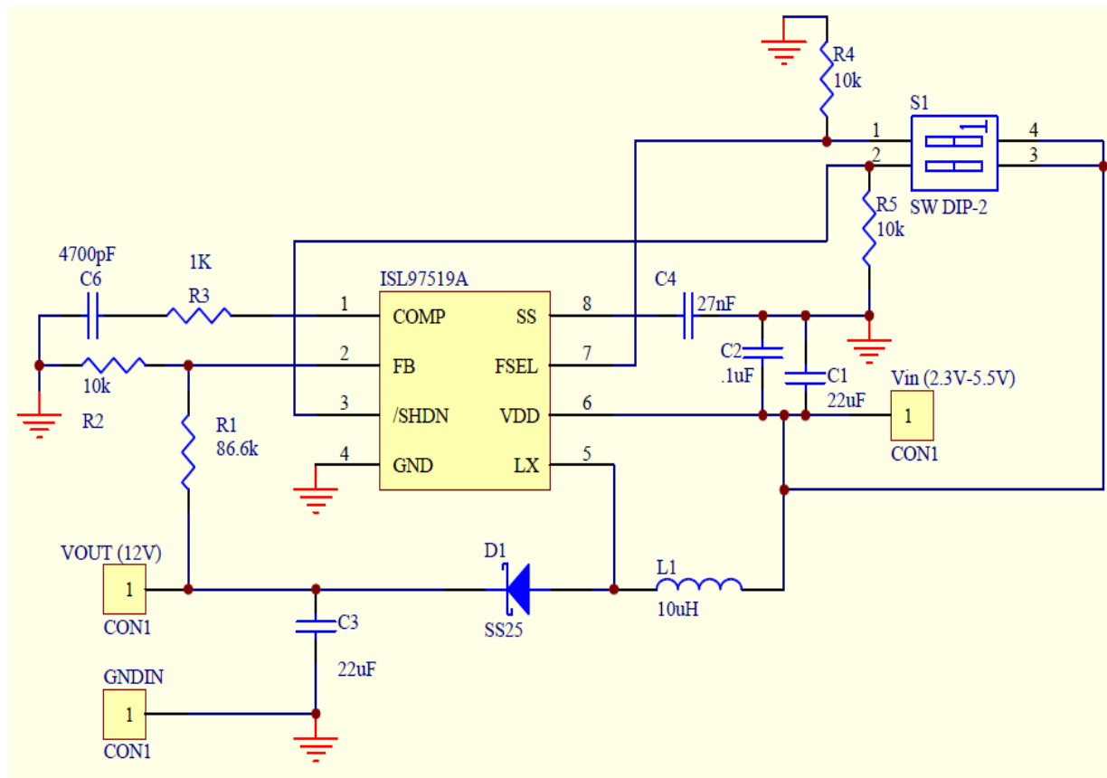
FIGURE 1. SCHEMATIC
