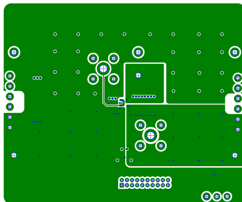
Figure 11. ISL9123xIIX-EVZ Inner Layer 3
