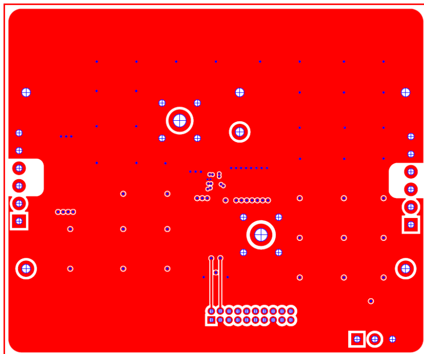
Figure 12. ISL9123xIIX-EVZ Bottom Layer Silk Screen
