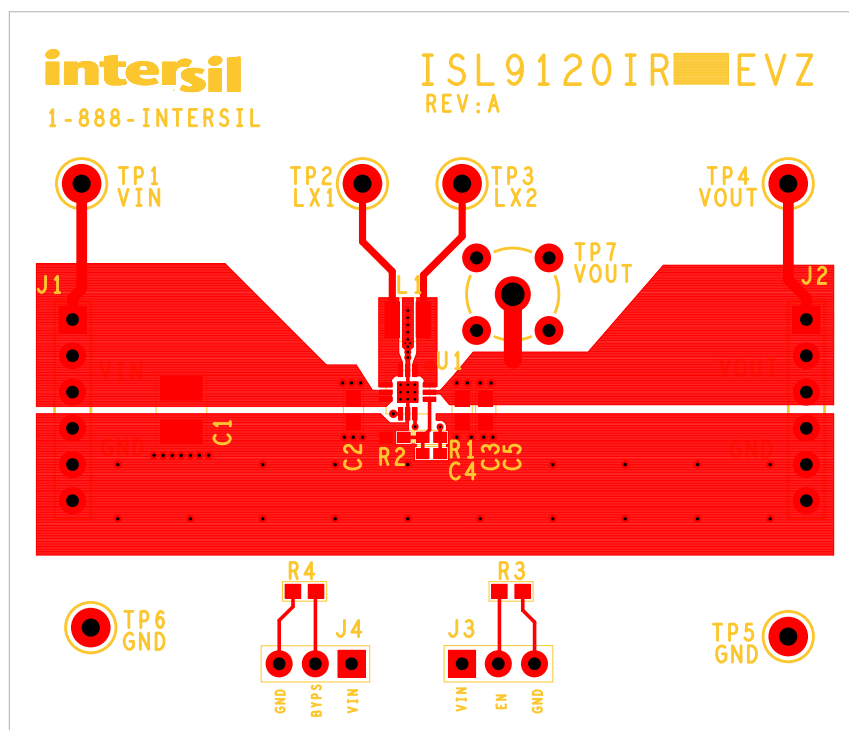
FIGURE 8. TOP LAYER
