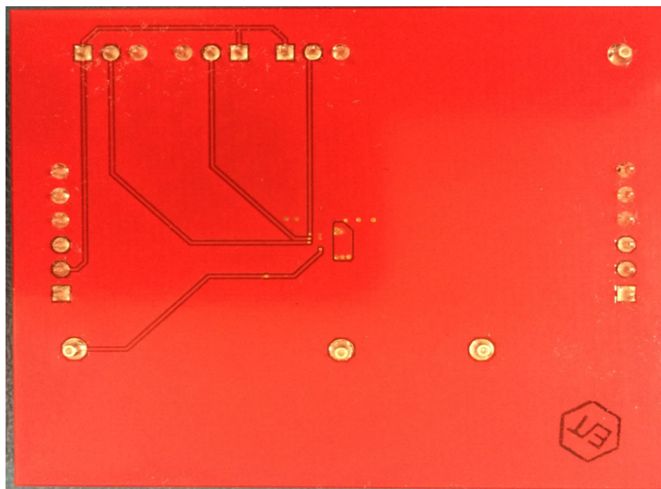
FIGURE 4. BOTTOM VIEW
