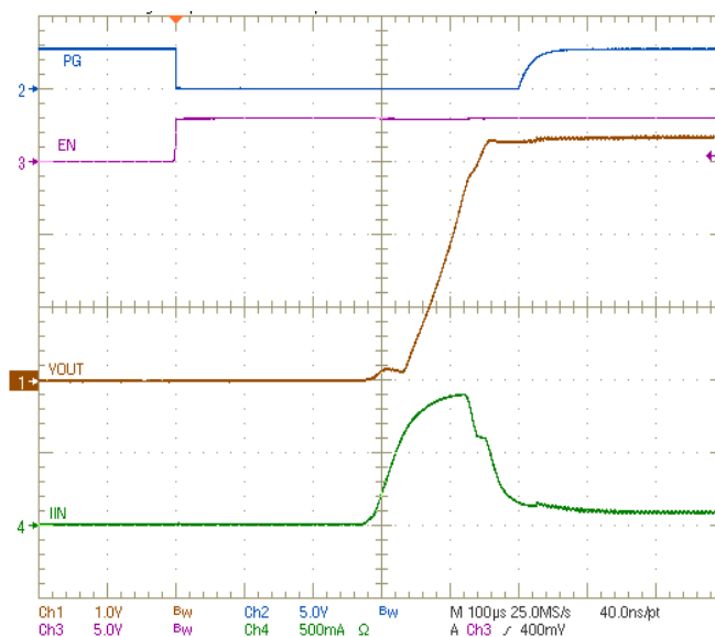
FIGURE 2. START-UP WAVEFORM 50Ω LOAD
