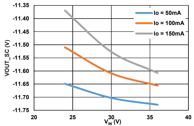
Figure 15. V_{OUT\_SC} Regulation vs V_{IN} , V_{OUT} = \pm 12V
