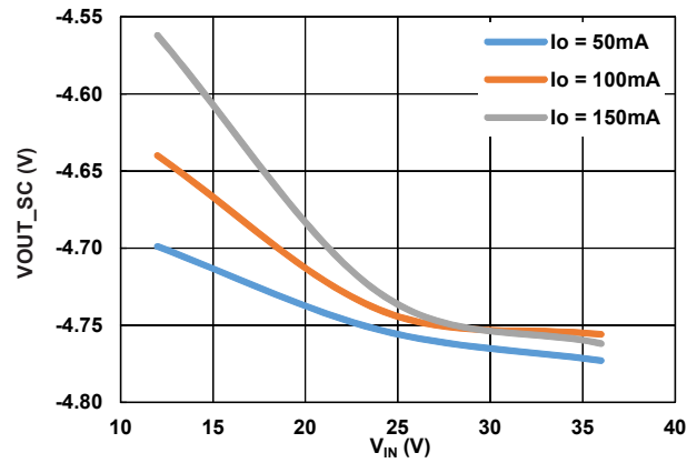
Figure 13. V_{OUT\_SC} Regulation vs V_{IN} , V_{OUT} = \pm 5V
