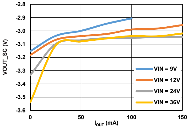
Figure 10. V_{OUT\_SC} Regulation vs I_{OUT} , V_{OUT} = \pm 3.3V
