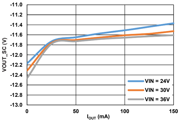
Figure 14. V_{OUT\_SC} Regulation vs I_{OUT} , V_{OUT} = \pm 12V
