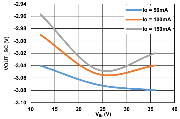
Figure 11. V_{OUT\_SC} Regulation vs V_{IN} , V_{OUT} = \pm 3.3V
