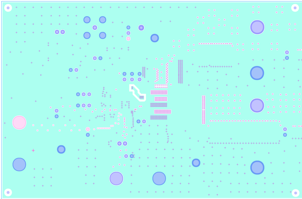
Figure 9. ISL73041SEHEV1Z Layer 3
