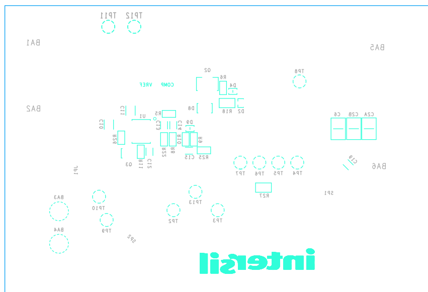
Figure 6. Bottom Silkscreen
