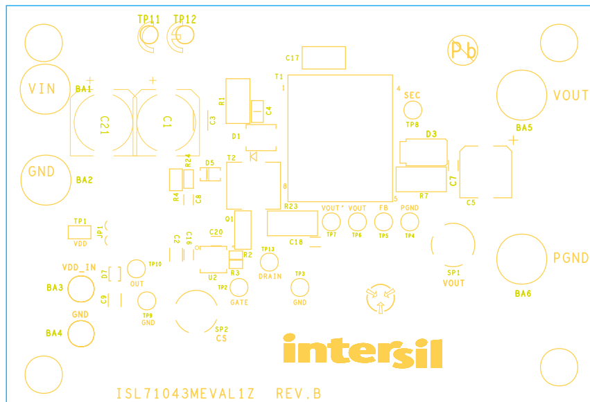
Figure 5. Top Silkscreen
