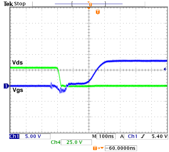
FIGURE 14. Q5 TURN ON, NO LOAD
