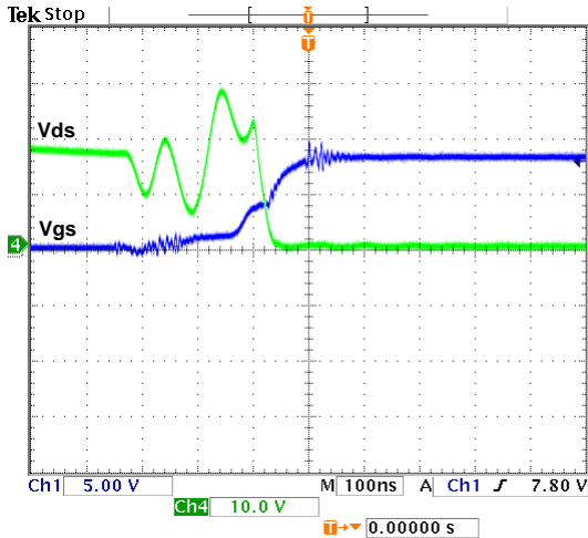
FIGURE 12. Q4 TURN ON, NO LOAD
