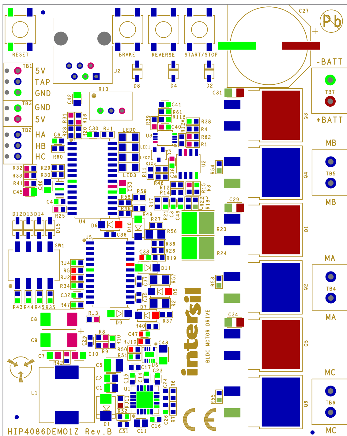
Figure 26. Silkscreen Top
