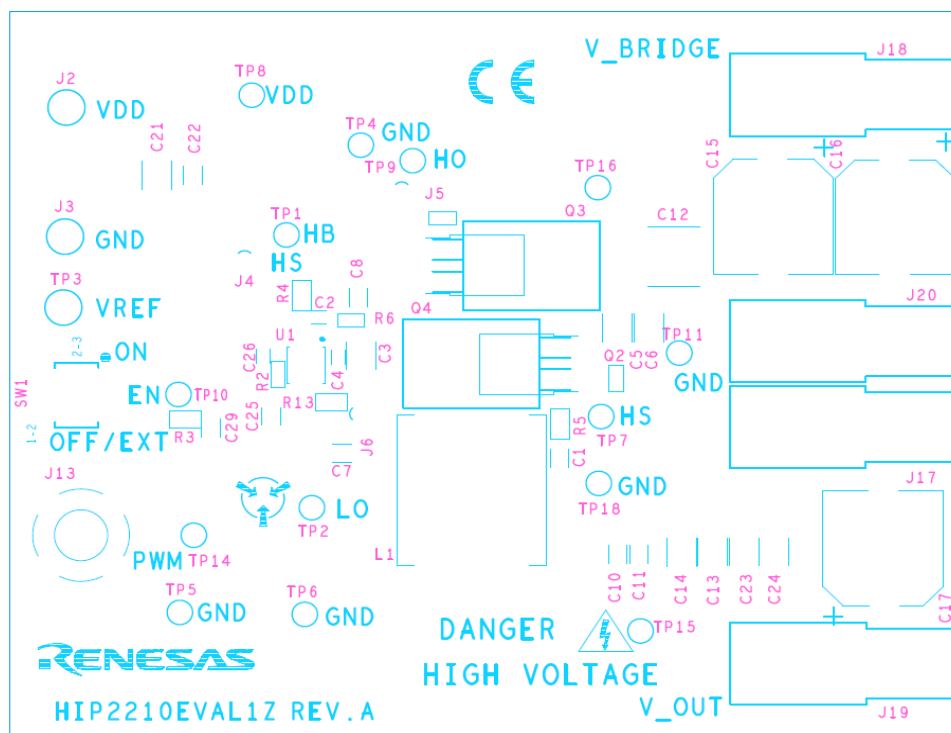
Figure 5. Silkscreen Top Layer
