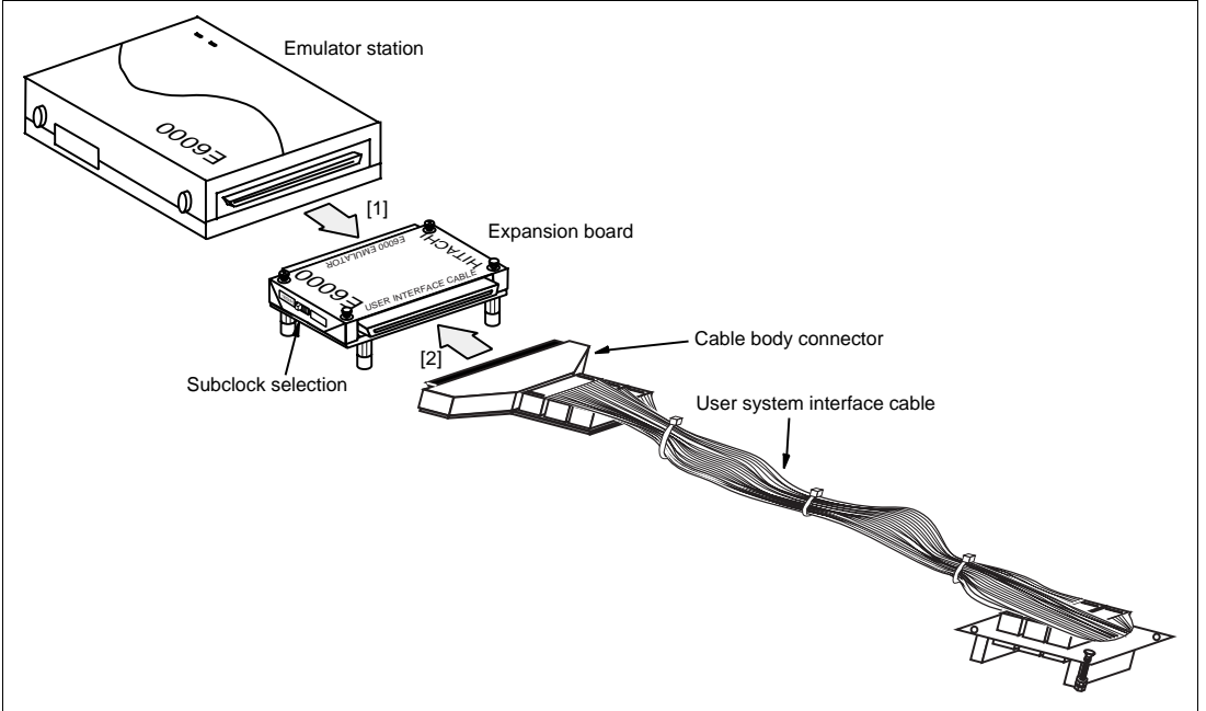
Figure 2 Connecting User System Interface Cable to Expansion Board
