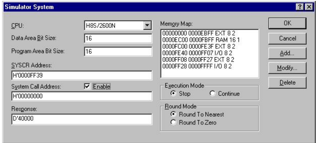
Figure 5.6 Simulator System Dialog Box
