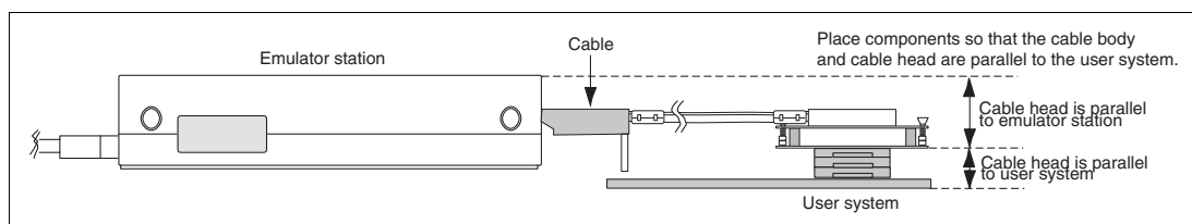
Figure 8 User System Interface Cable Location Example
