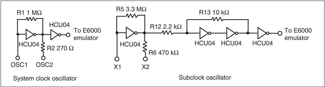
Figure 7 System Clock Oscillator Circuit
