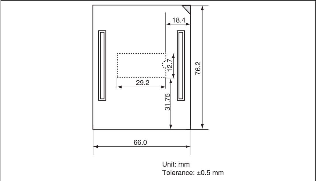
Figure 5 Dimensions for User System Interface Cable Head
