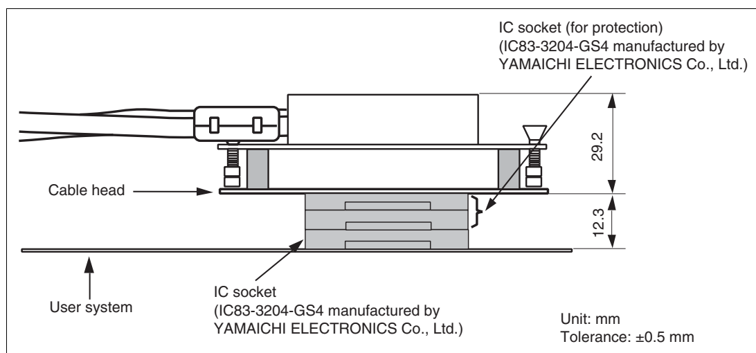
Figure 6 Resulting Dimensions after Connecting User System Interface Cable
