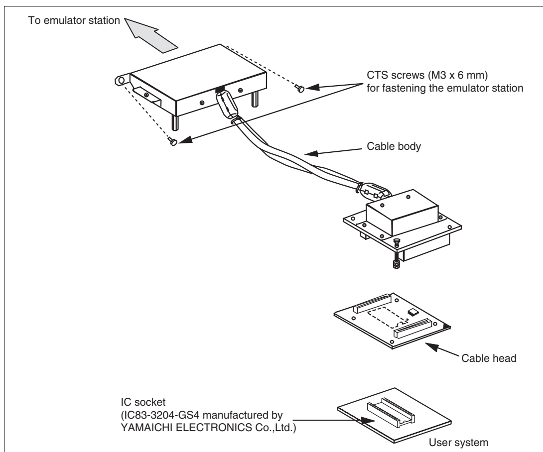
Figure 1 HS36902ECS61H User System Interface Cable
