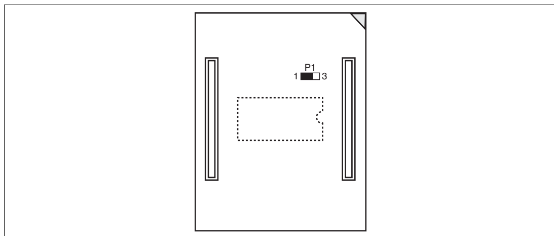
Figure 9 P1 Short Connector
