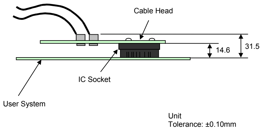
Figure 3.3 Connecting user system interface cable to user system
