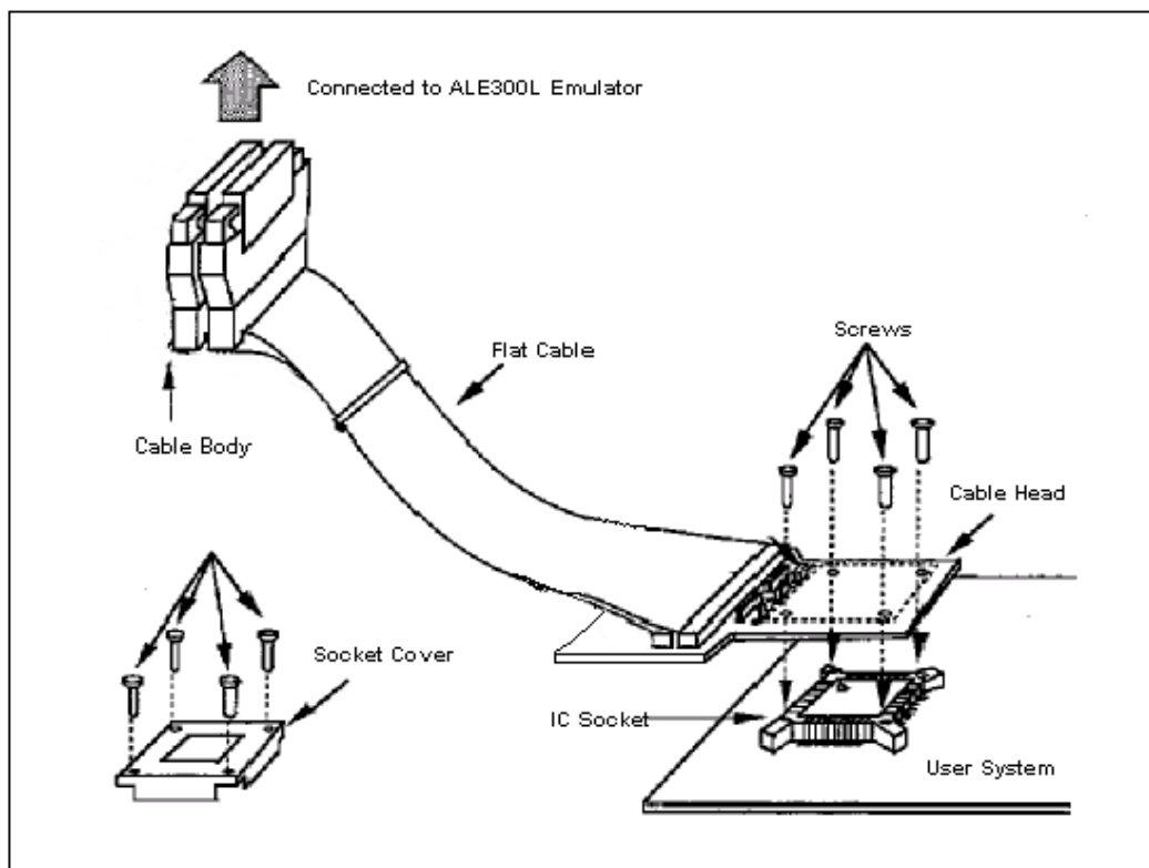
Figure 1.1 SD99AC3887TA0G user system interface cable
