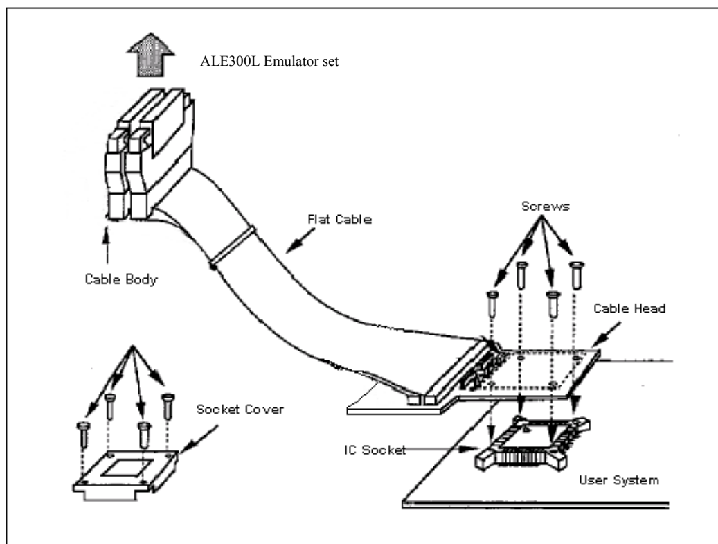
Figure 1.1 SD00AC3802F64A user system interface cable
