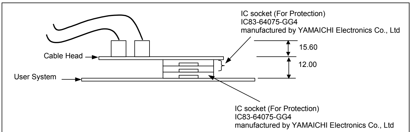
Figure 3.3 Connecting user system interface cable to user system
