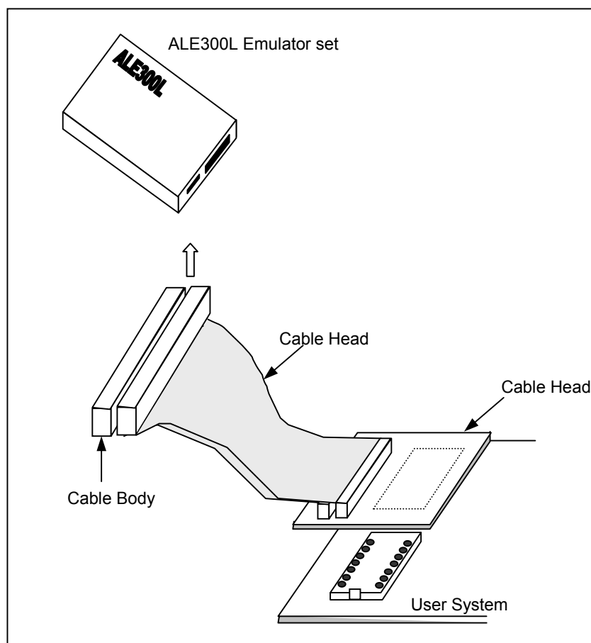
Figure 2.1 Connect User System Interface Cable to ALE300L Emulator
