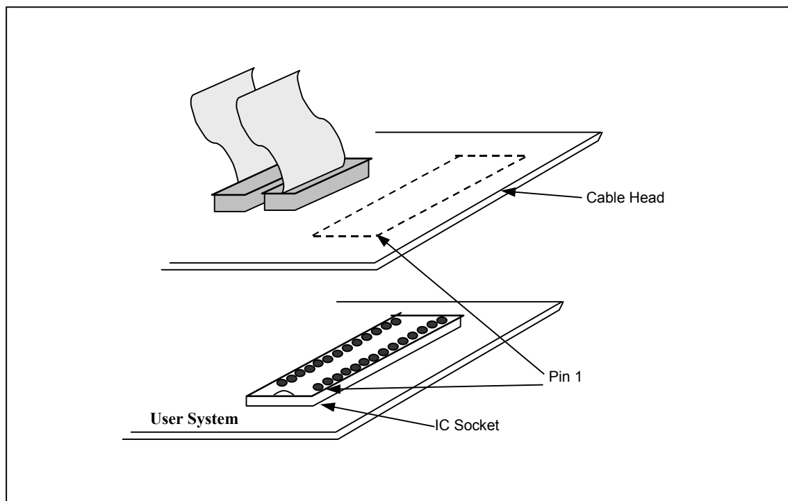
Figure 2.2 Connecting user system interface cable to user system
