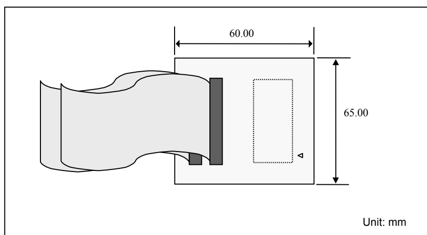
Figure 3.2 User system interface cable head
