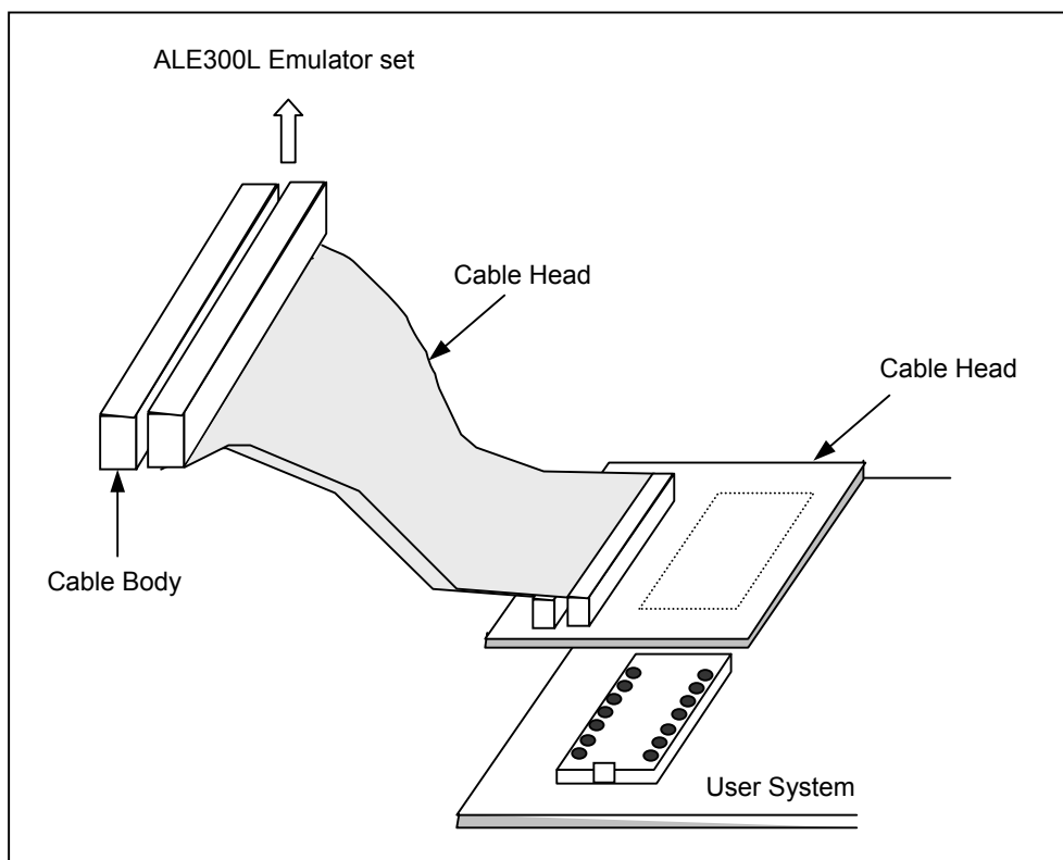
Figure 1.1 SD01AC3802D64S user system interface cable
