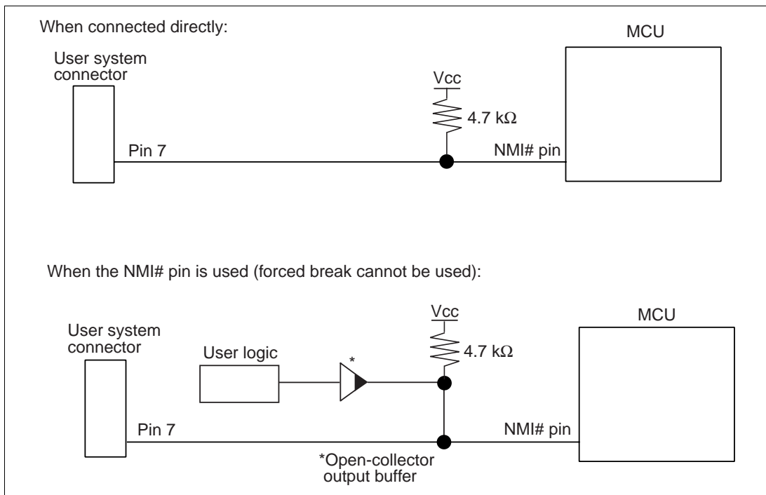
Figure 3.4 Connection of Emulator and NMI# Pin
