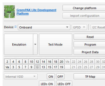
Figure 9. Debugging Setup for DIP and Socket Adapters
