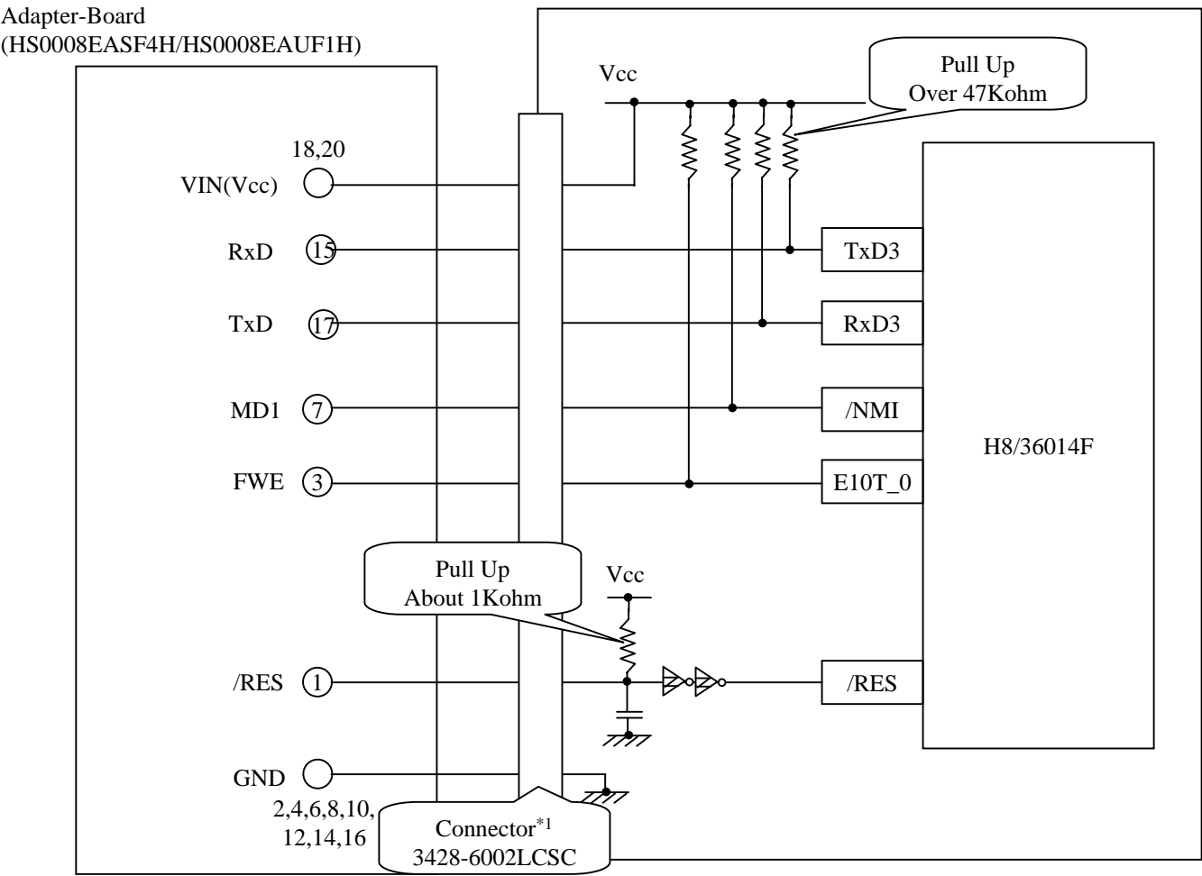
Setting the switches on the HS0008EASF4H on using H8/36014F *1:Sumitom 3M,Ltd
