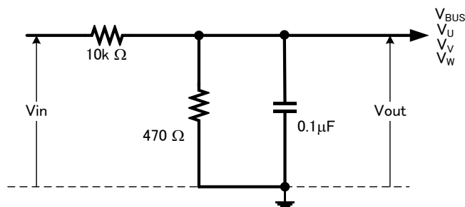
Figure 6-4 Output Voltage Detection Circuit
