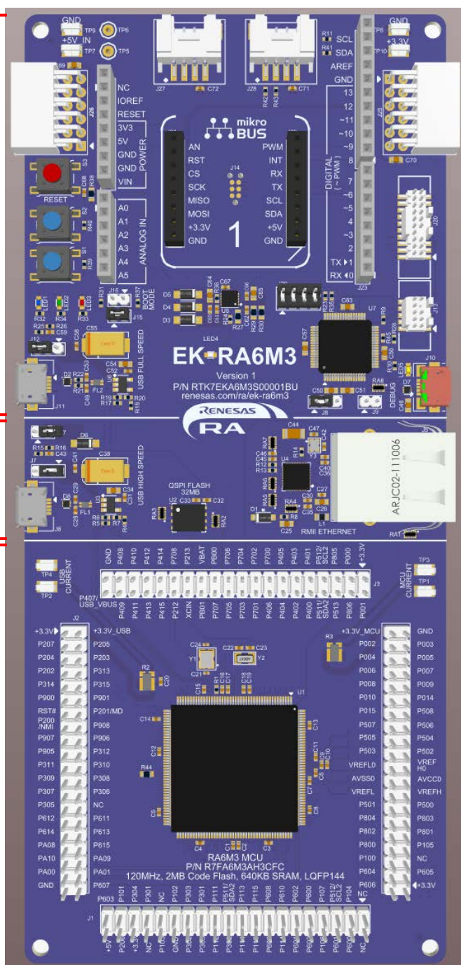
Figure 4. EK-RA6M3 Board Functional Area Definitions
